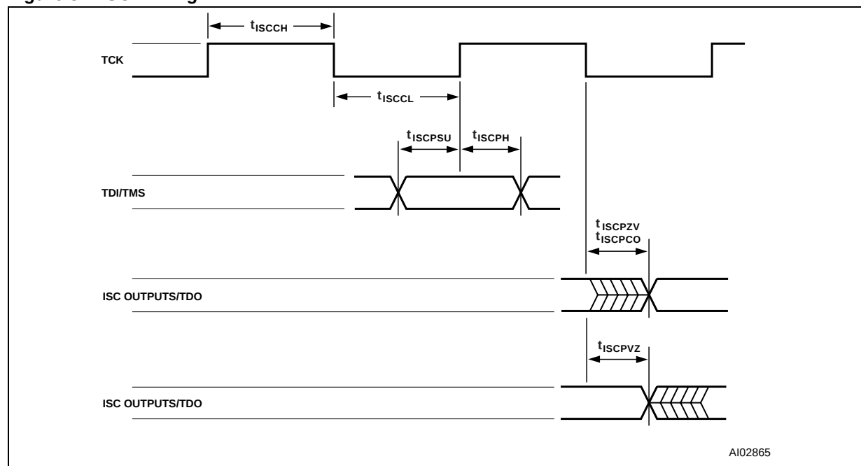
Figure 37. ISC Timing
