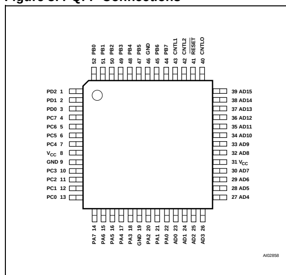
Figure 3. POFP Connections
